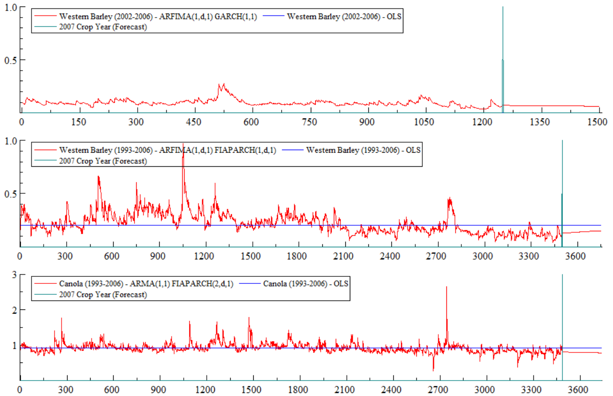
Figure 3. FIAPARCH/GARCH and OLS hedge ratios
